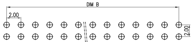
PCB LAYOUT
