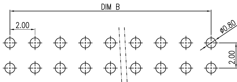
PCB LAYOUT
