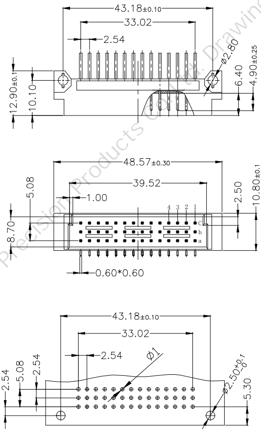
PCB LAYOUT(RECOMMENDED) (TOP VIEW TOL. :±0.05)
