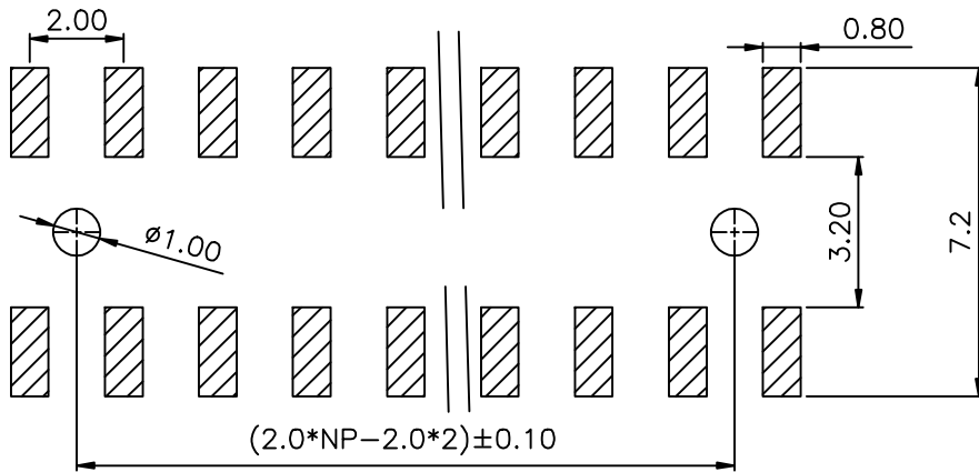
PCB LAYOUT
