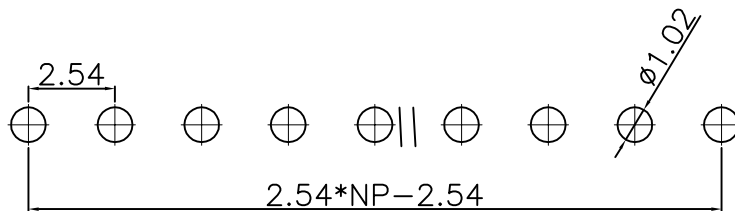
PCB LAYOUT
